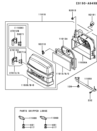
B-11 AIR-FILTER/MUFFLER
