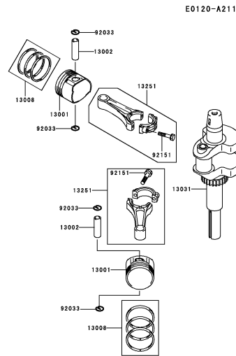
B-04 PISTON/CRANKSHAFT
