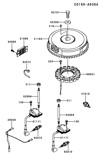
B-08 ELECTRIC-EQUIPMENT
