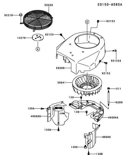
B-07 COOLING-EQUIPMENT
