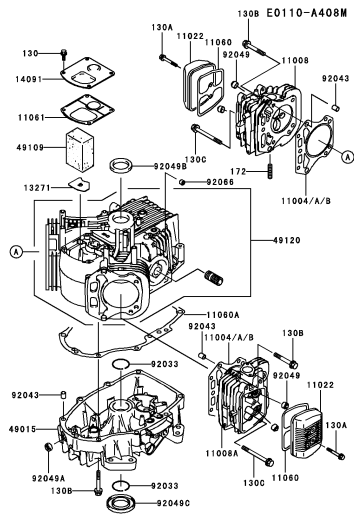
B-03 CYLINDER/CRANKCASE
