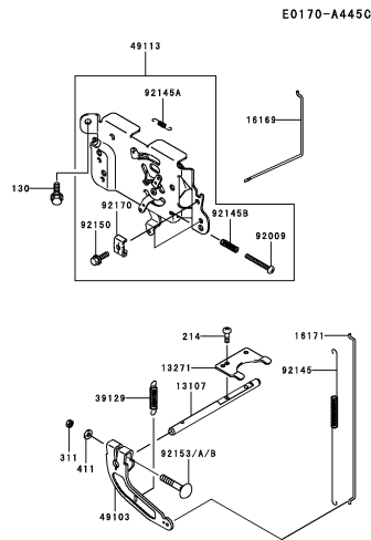
B-09 CONTROL-EQUIPMENT
